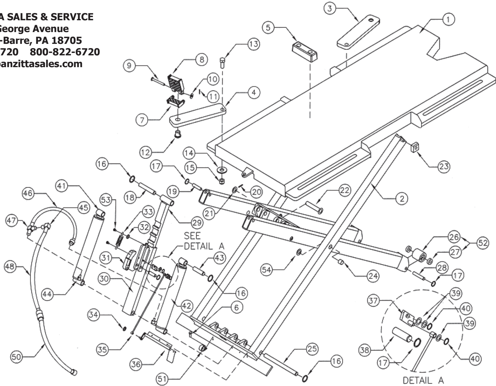
10.1 MIDRISE MAIN FRAME ASSEMBLY
