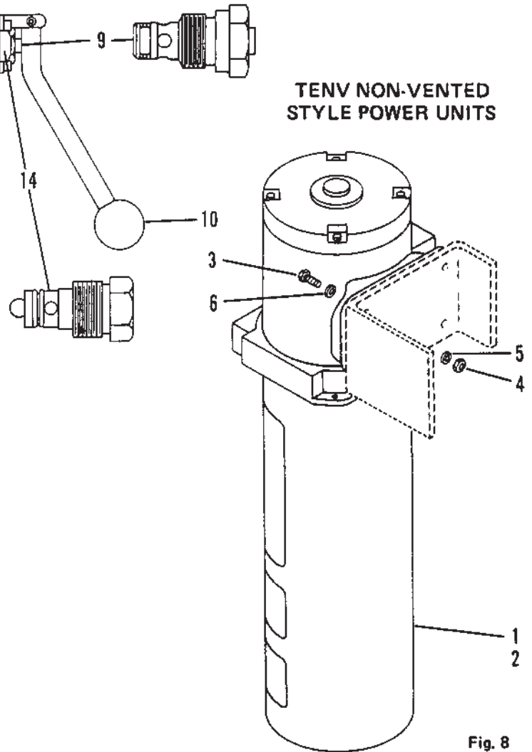
POWER UNIT
