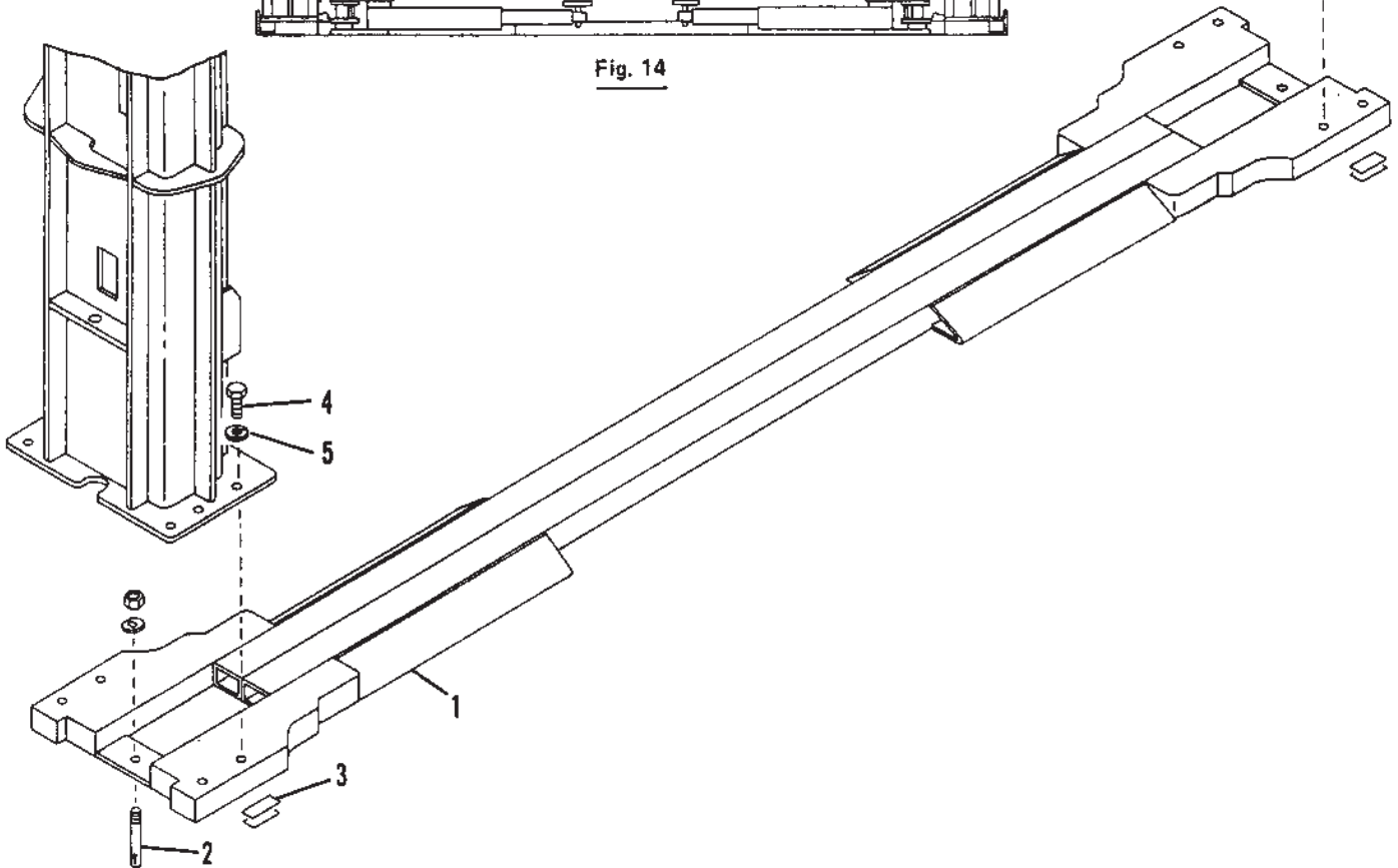
BASE ASSEMBLY
