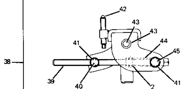
BOTTOM ADAPTER TK-600-1
