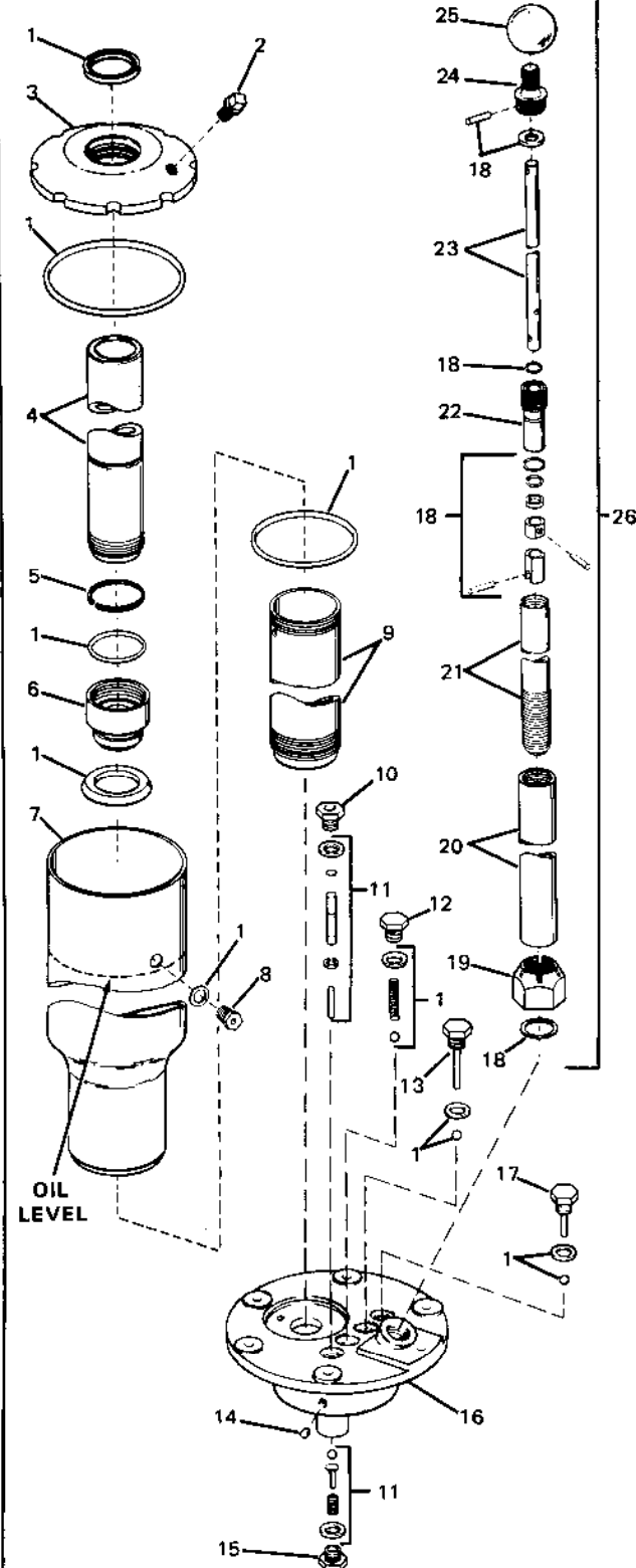
HYDRAULIC POWER UNIT K372.900
